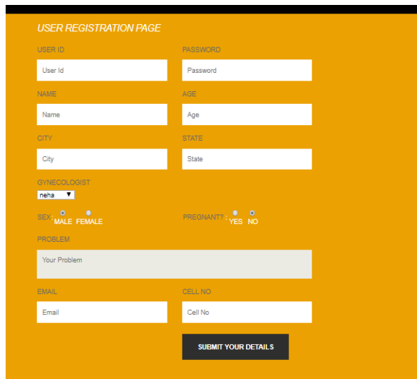
Fig. 3: Registration page
